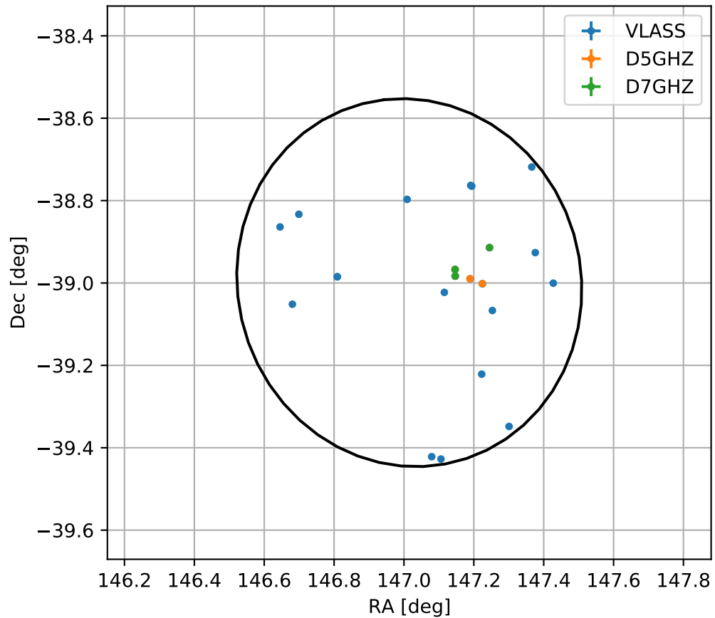
4FGL J0948.0-3859
