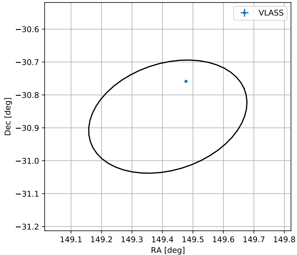
4FGL J0957.6-3051
