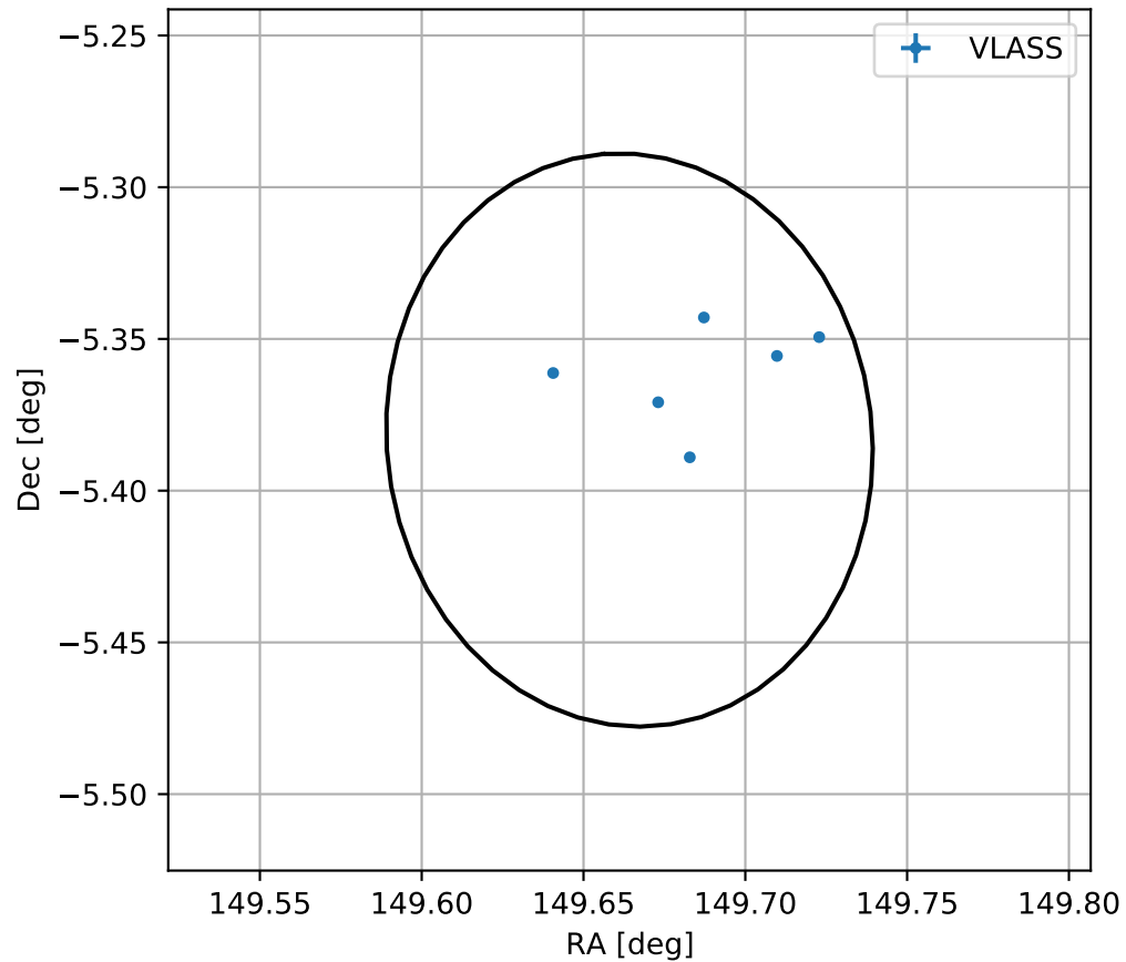
4FGL J0958.6-0522
