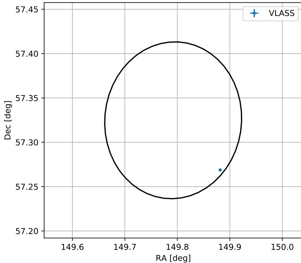
4FGL J0959.1+5719
