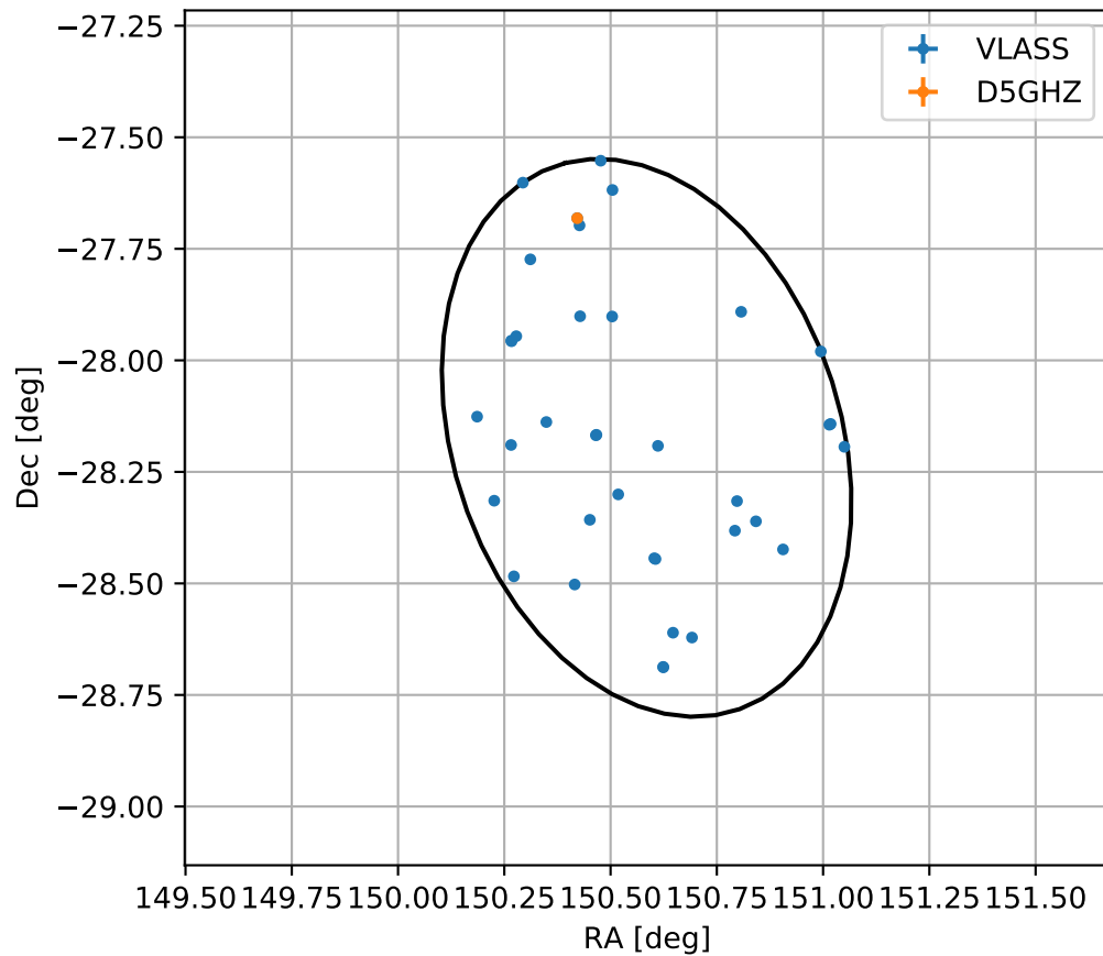
4FGL J1002.3-2810
