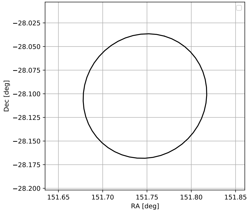
4FGL J1006.9-2806
