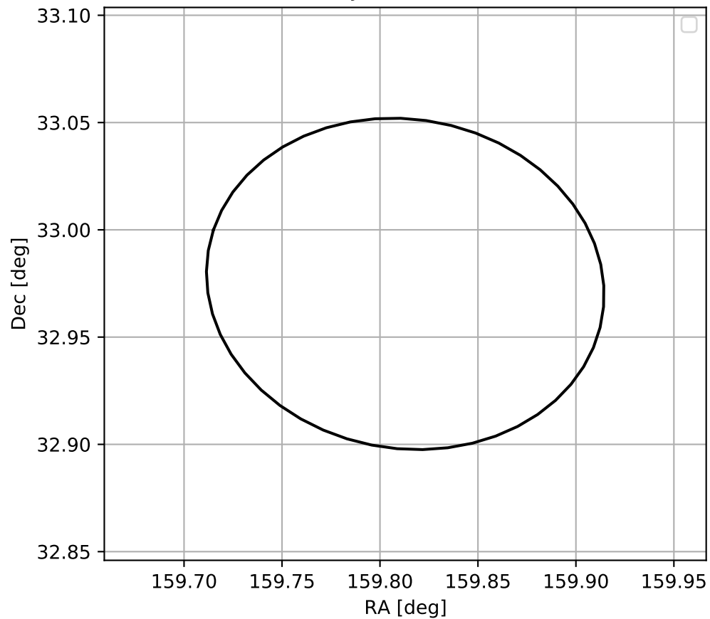
4FGL J1039.2+3258
