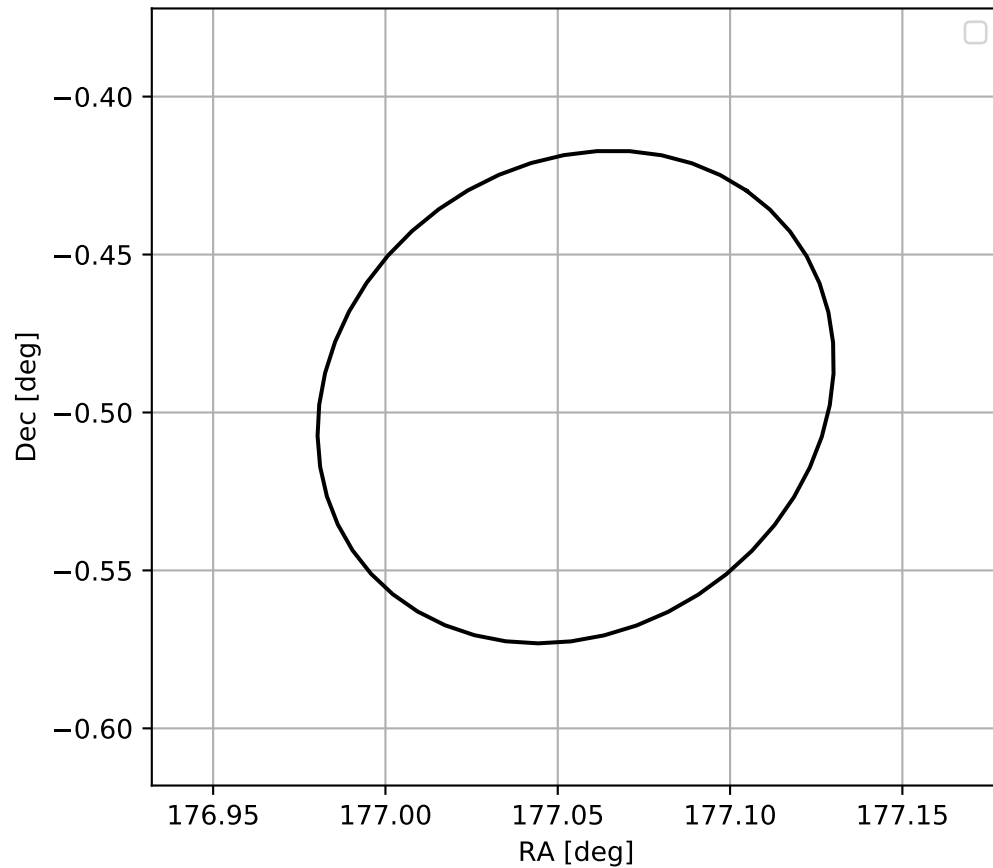
4FGL J1148.2-0029
