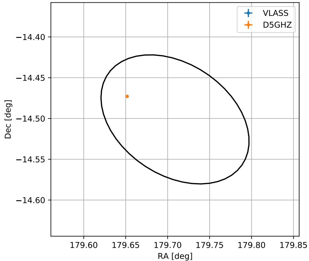
4FGL J1158.8-1430
