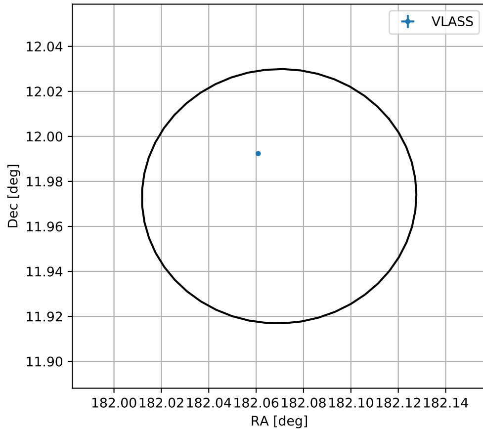
4FGL J1208.2+1158
