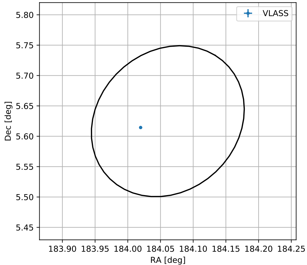
4FGL J1216.2+0537
