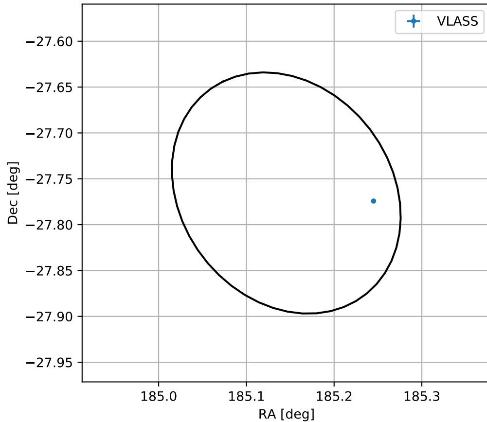
4FGL J1220.5-2745
