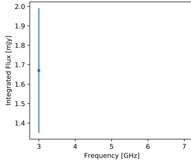
F357 J125652.21-133501.6 (unr)
