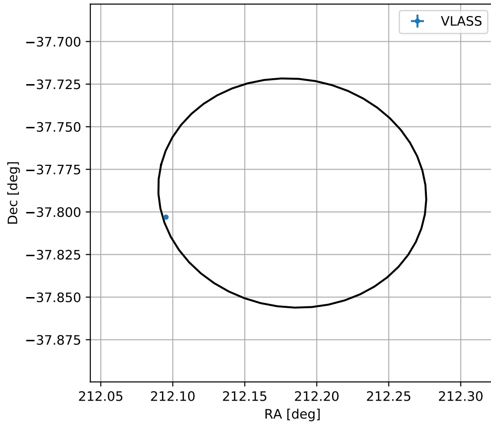
4FGL J1408.7-3747
