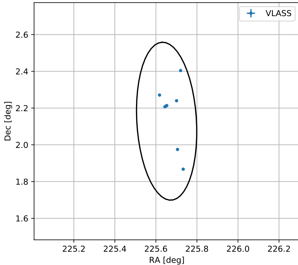
4FGL J1502.6+0207
