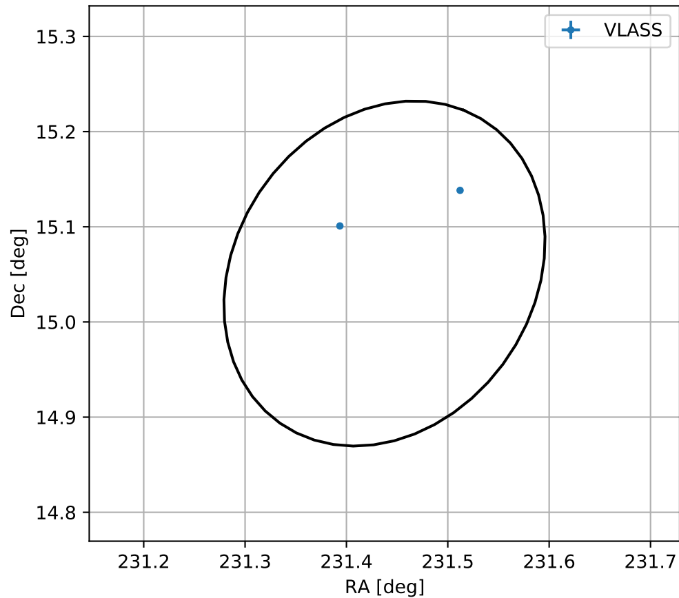
4FGL J1525.7+1503
