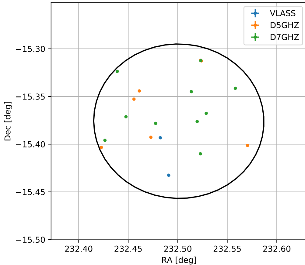
4FGL J1530.0-1522
