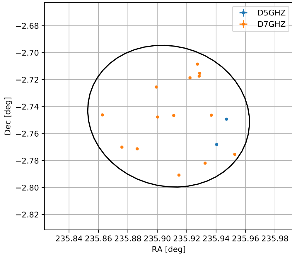
4FGL J1543.6-0244
