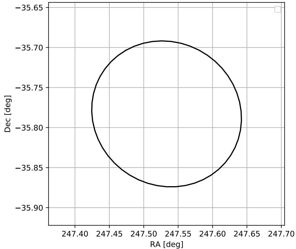
4FGL J1630.1-3546
