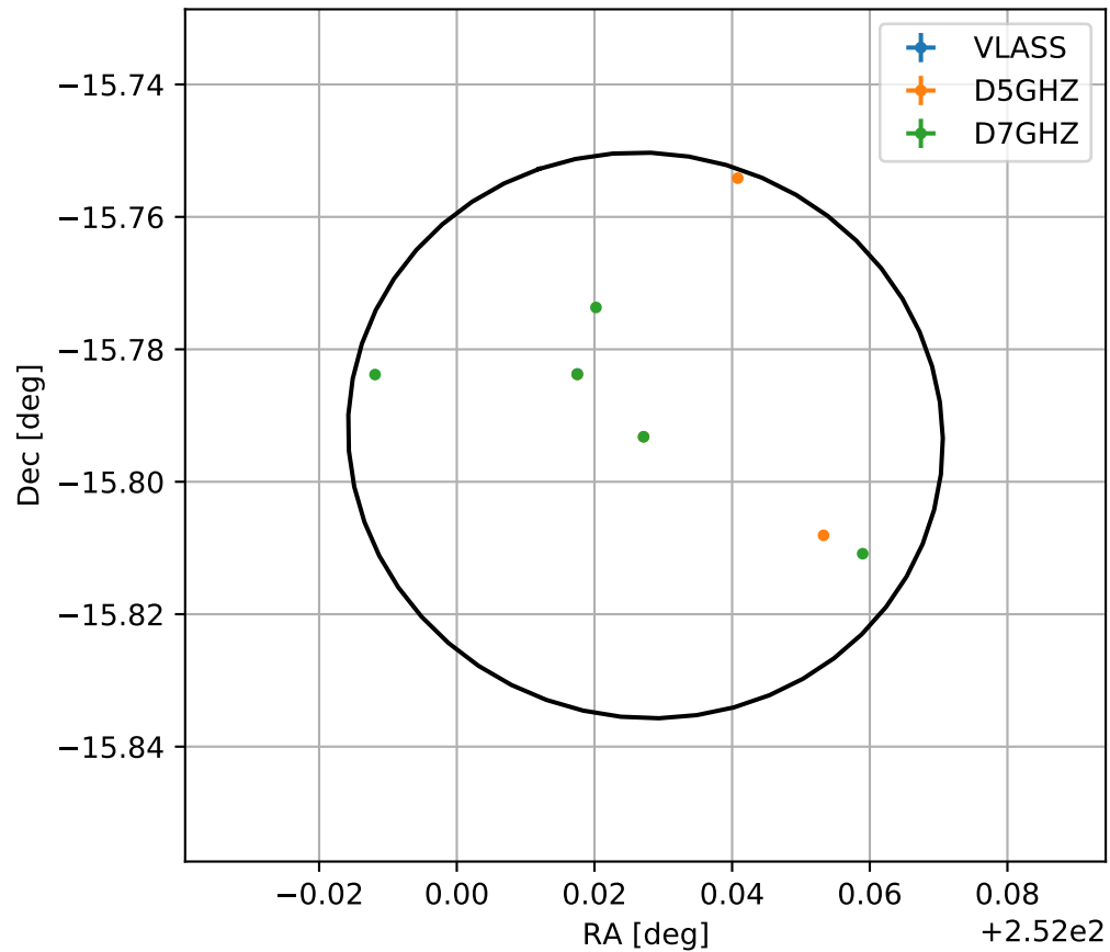
4FGL J1648.1-1547
