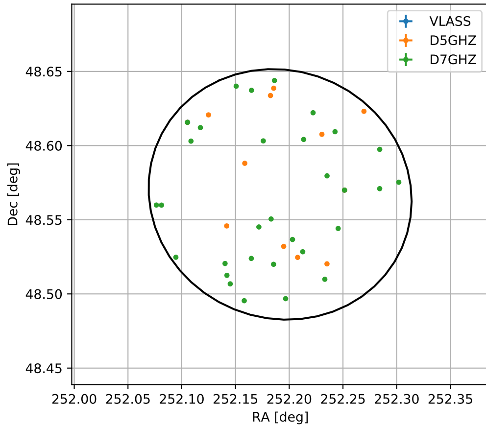
4FGL J1648.7+4834
