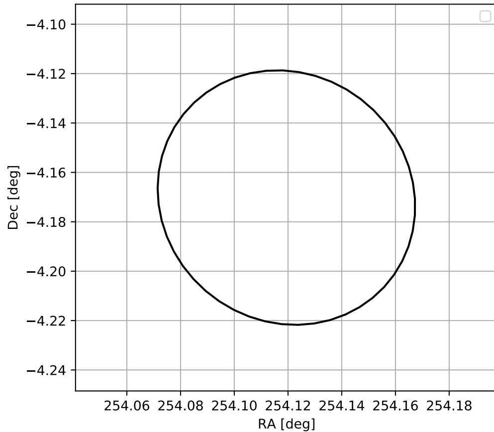
4FGL J1656.4-0410
