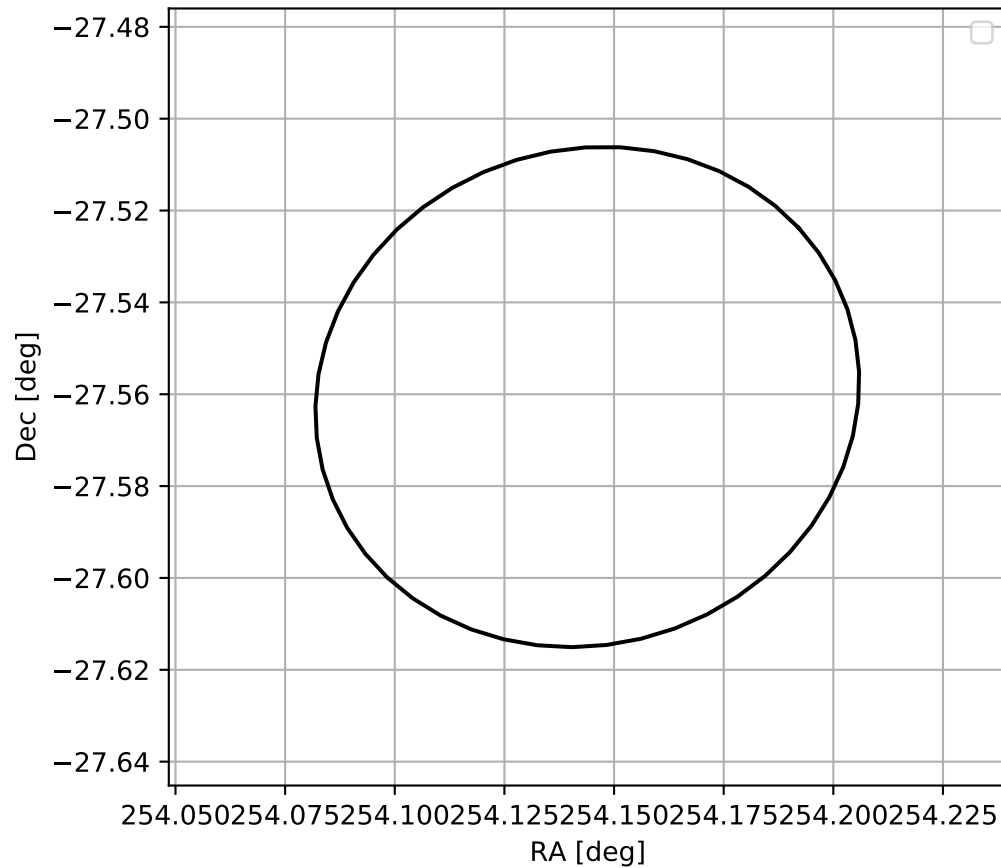
4FGL J1656.5-2733
