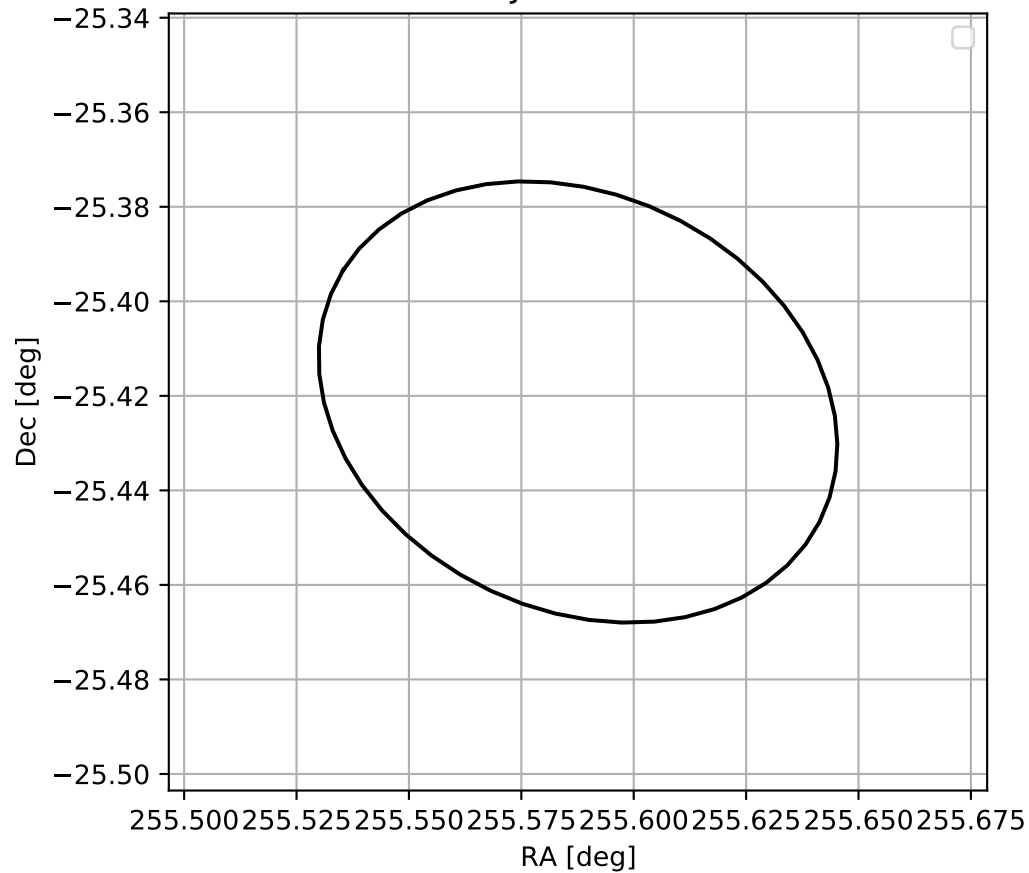
4FGL J1702.3-2525
