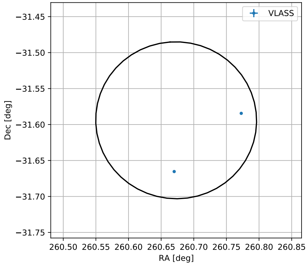
4FGL J1722.6-3135
