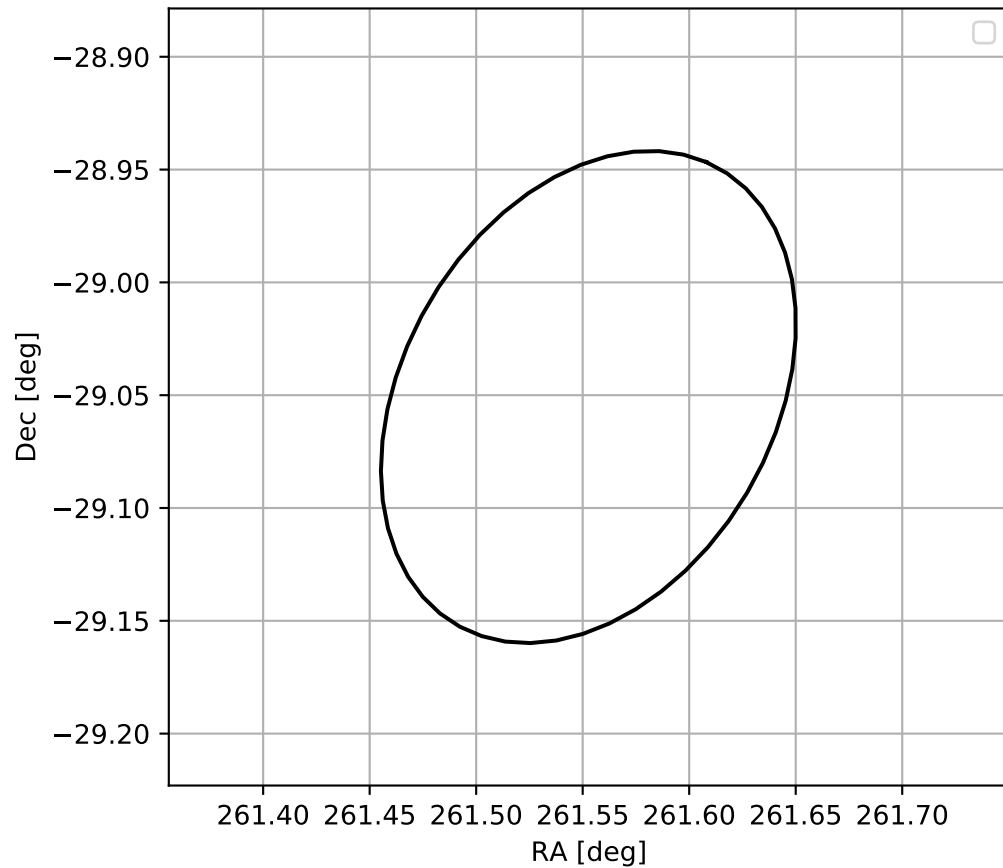
4FGL J1726.2-2903
