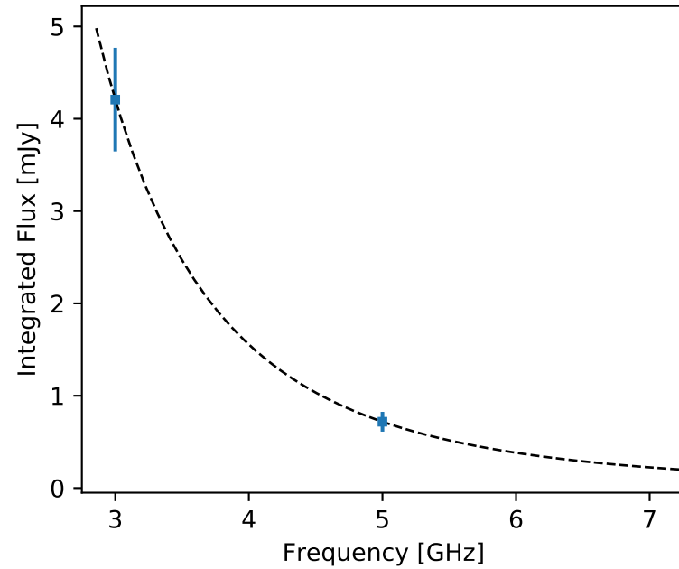
F357 J172646.35-270338.1 (unr)
