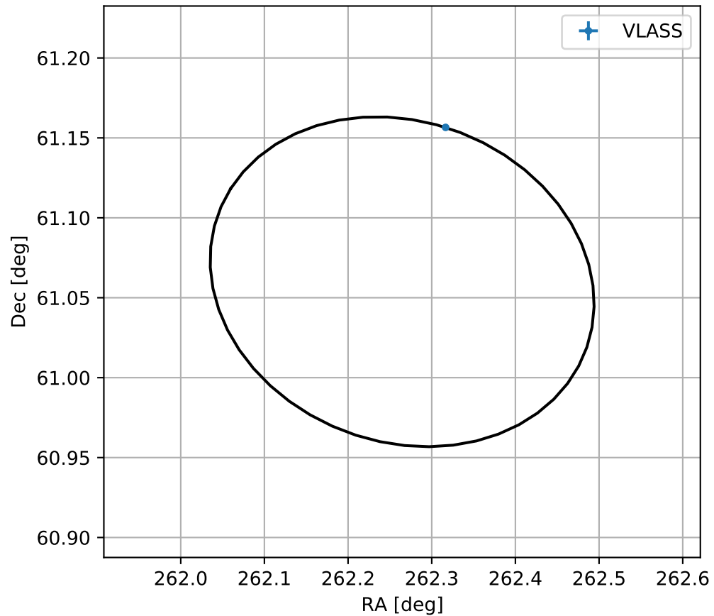
4FGL J1729.0+6103
