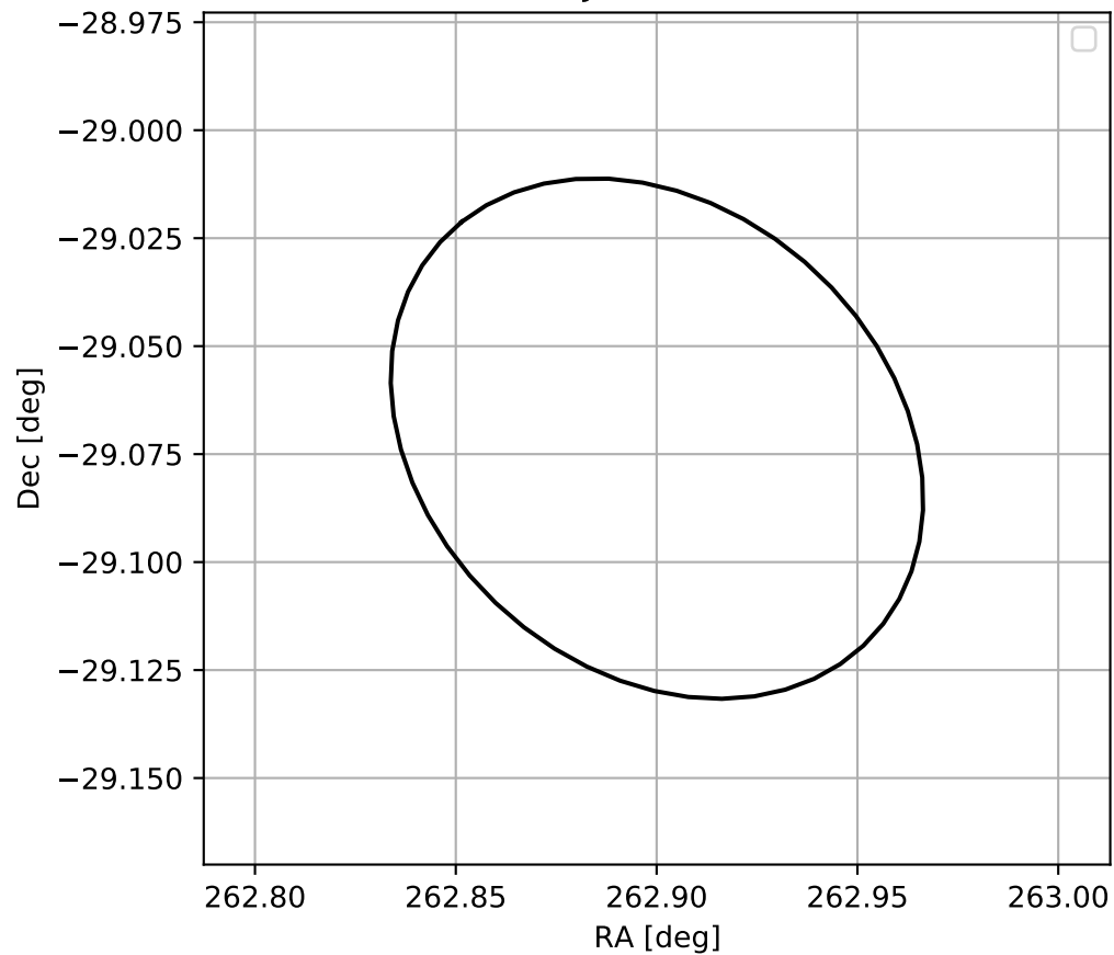
4FGL J1731.6-2904
