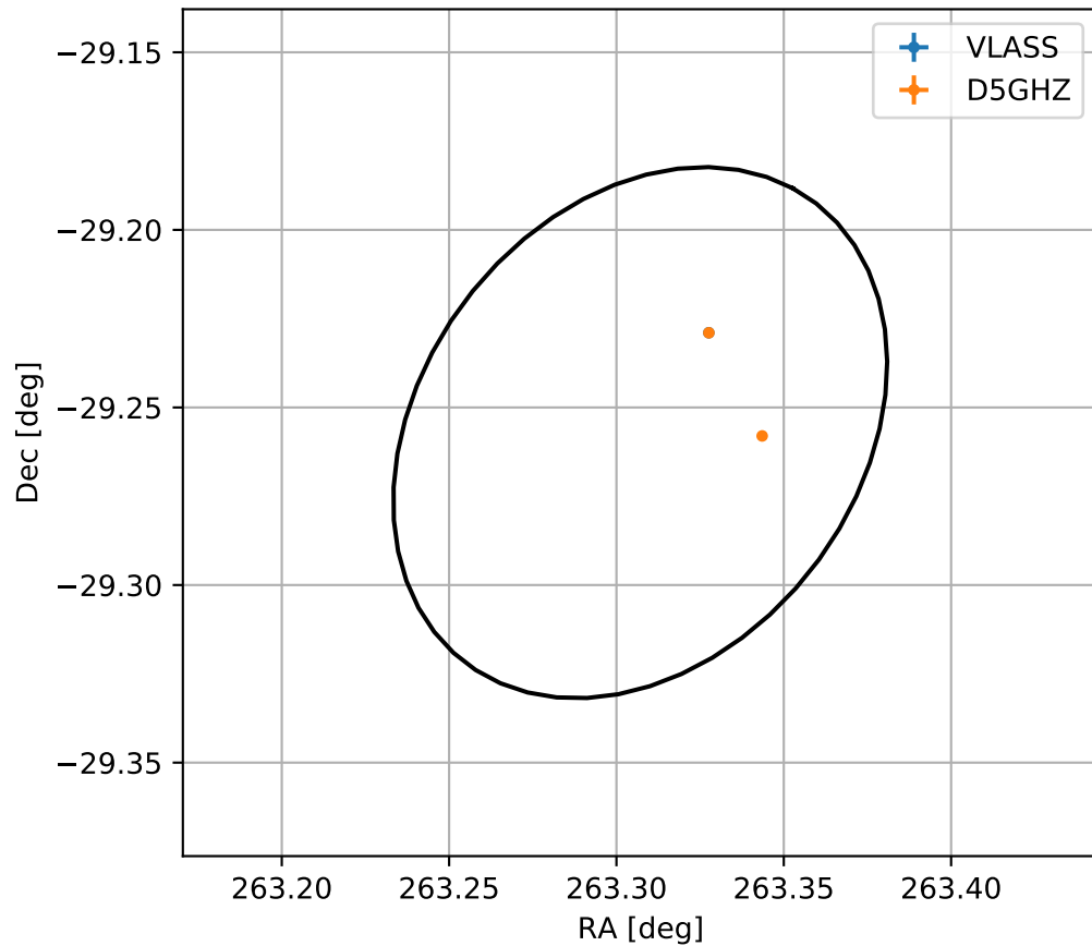
4FGL J1733.2-2915
