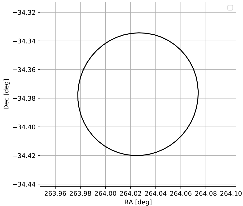
4FGL J1736.1-3422
