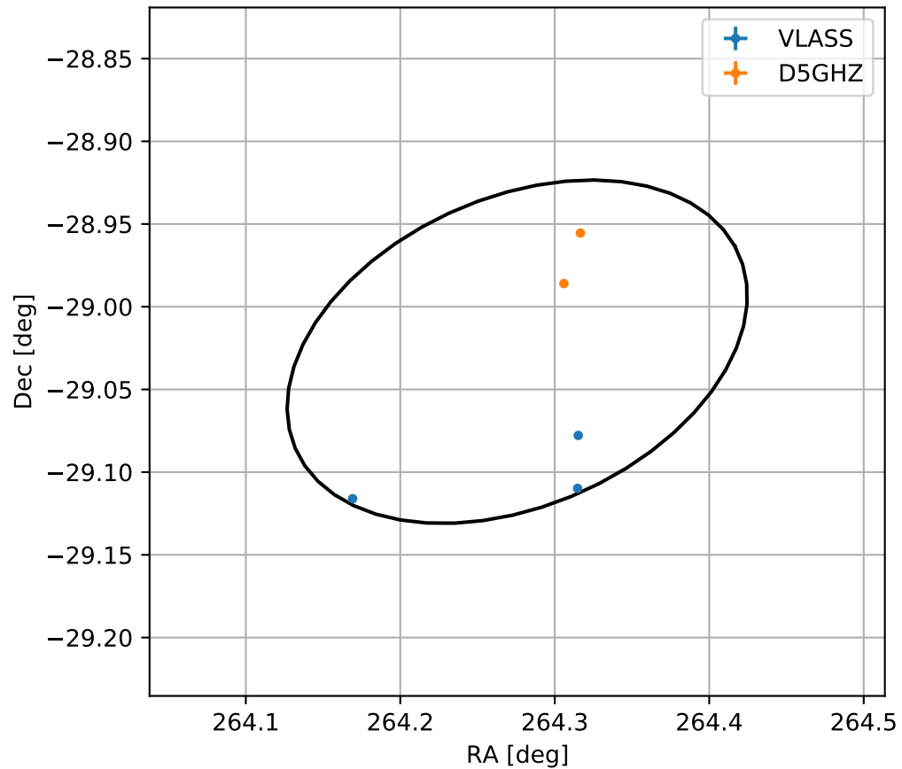
4FGL J1737.1-2901
