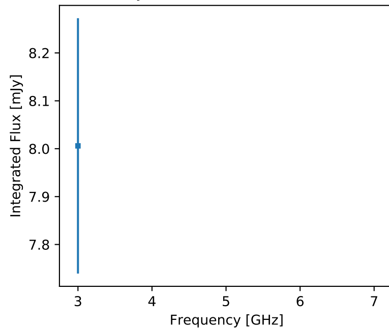
F357 J173721.16-242303.7 (unr)
