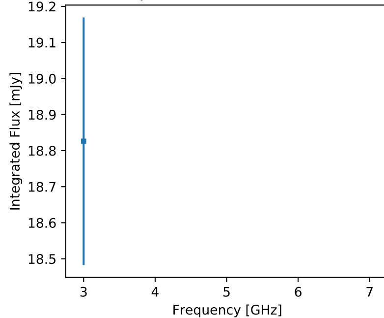
F357 J173721.16-242303.7 (unr)
