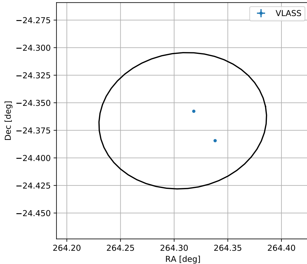
4FGL J1737.2-2421
