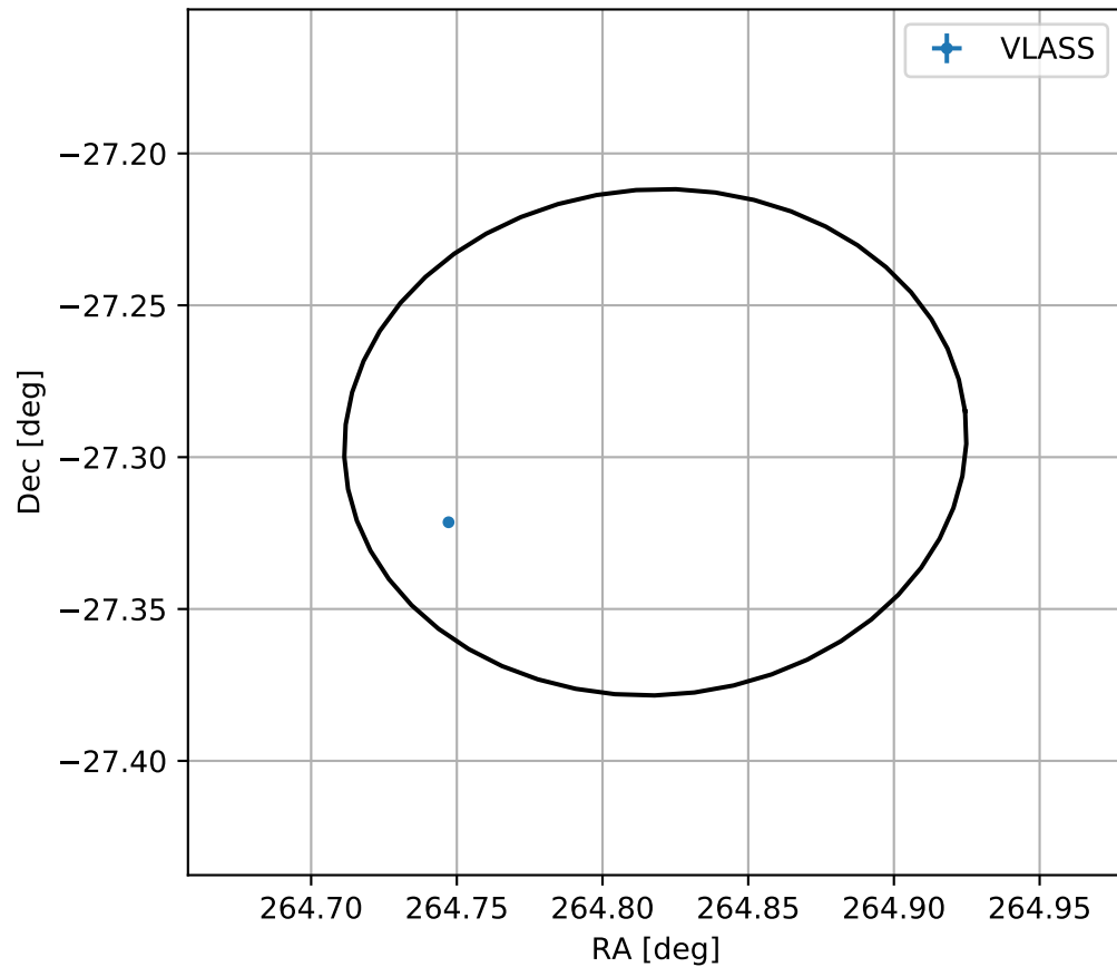
4FGL J1739.2-2717
