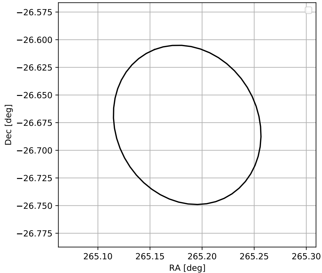
4FGL J1740.7-2640
