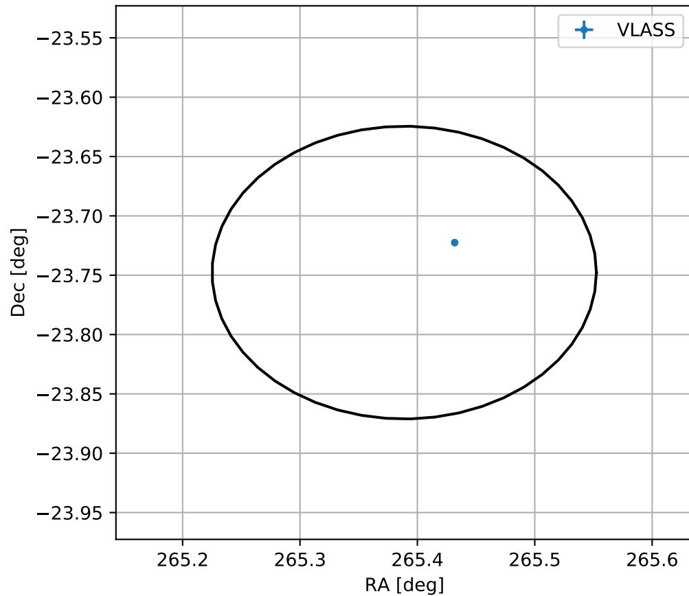
4FGL J1741.5-2344
