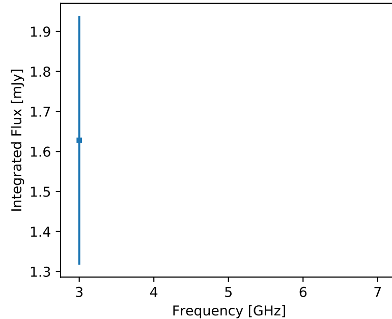
F357 J174239.62-284143.5 (unr)
