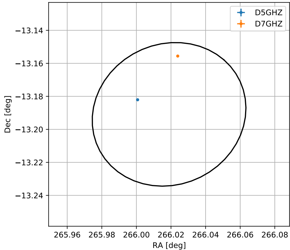
4FGL J1744.0-1311
