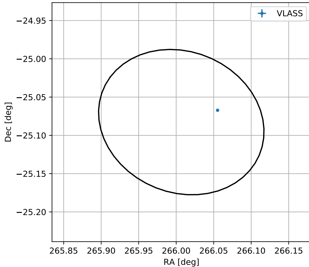
4FGL J1744.0-2504
