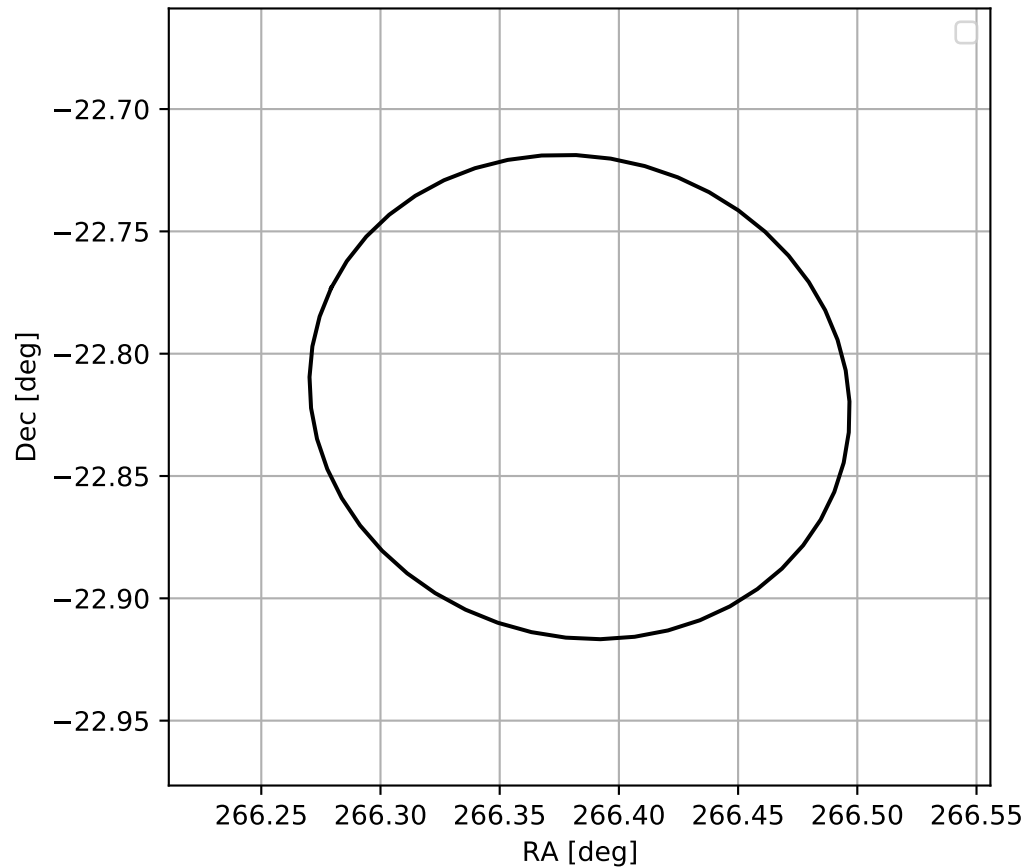
4FGL J1745.5-2249
