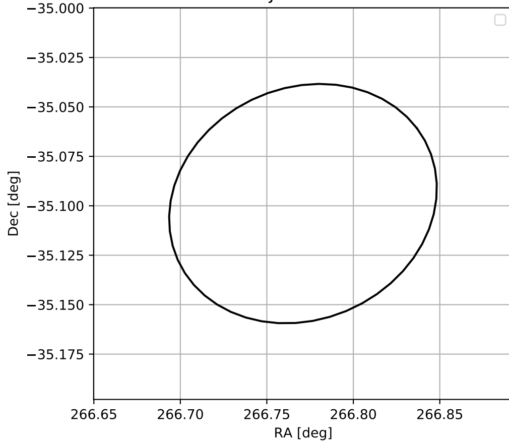
4FGL J1747.0-3505
