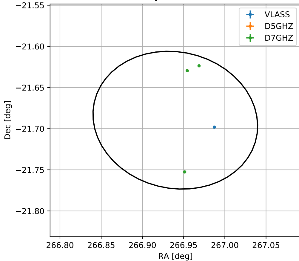
4FGL J1747.7-2141
