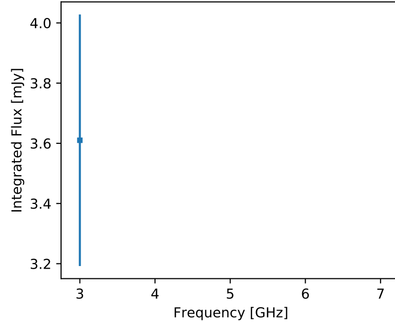
F357 J174927.14-314632.2 (unr)
