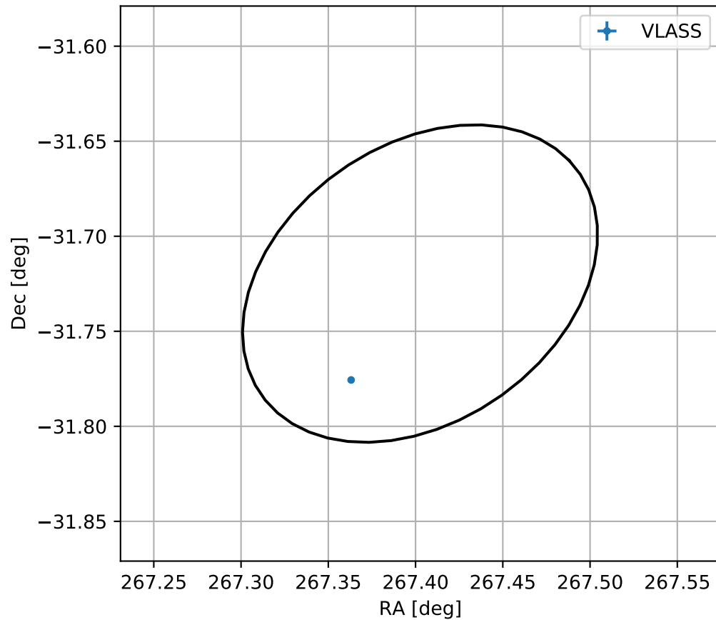
4FGL J1749.6-3143c
