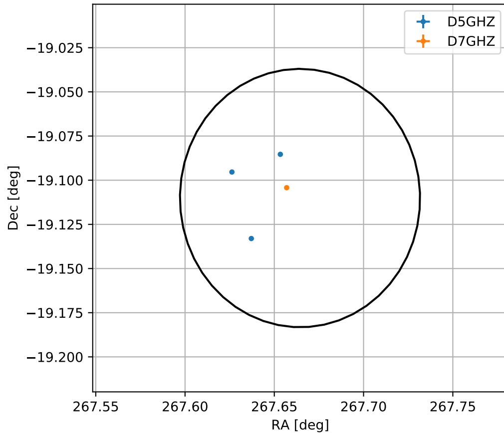
4FGL J1750.6-1906
