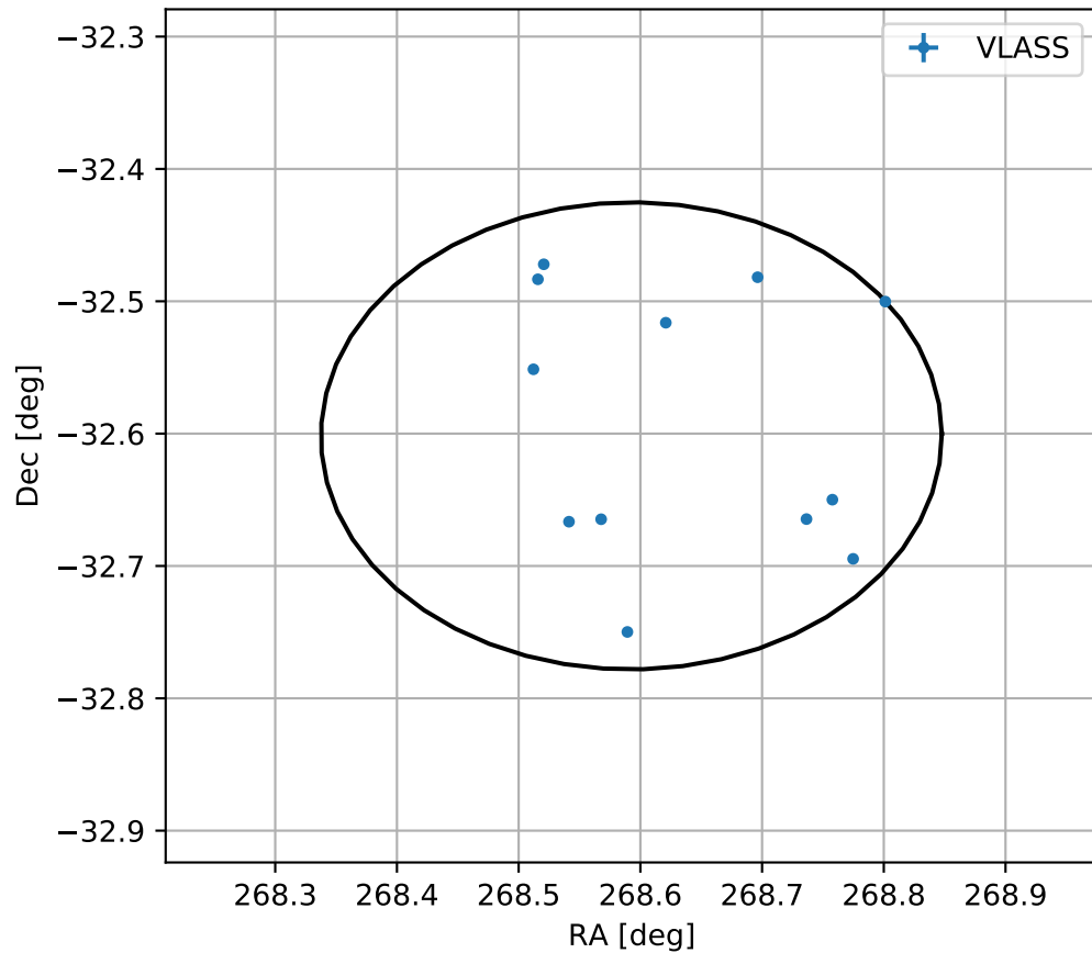
4FGL J1754.3-3236
