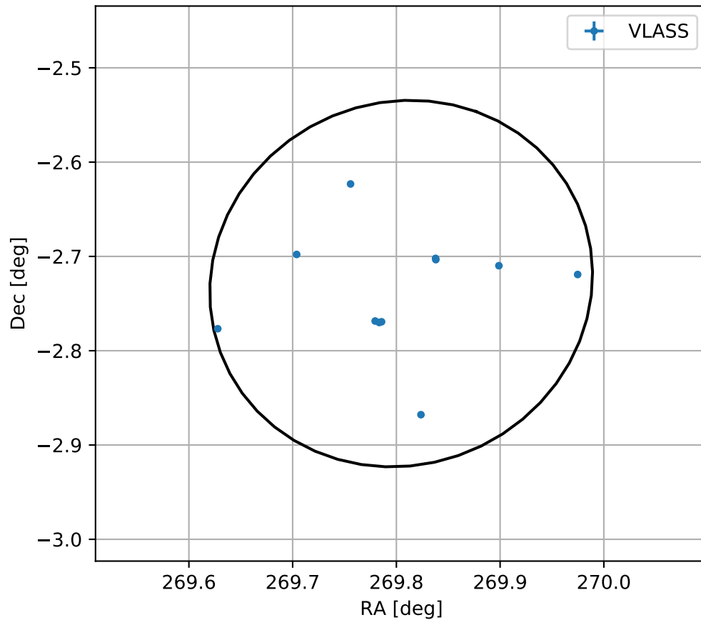
4FGL J1759.2-0243
