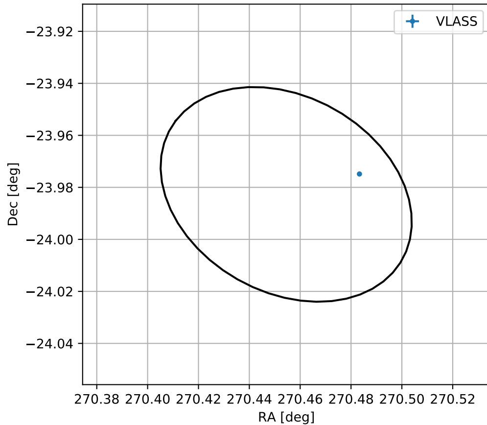
4FGL J1801.8-2358
