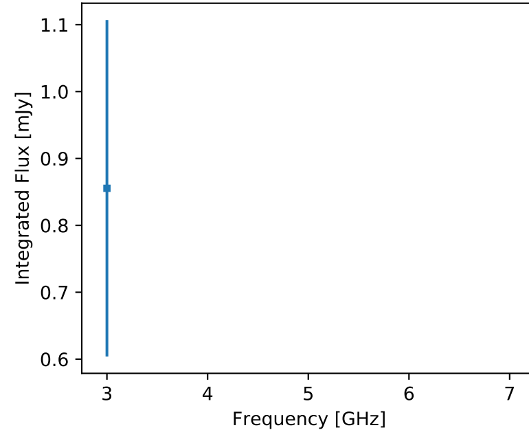
F357 J180202.01-264721.1 (unr)
